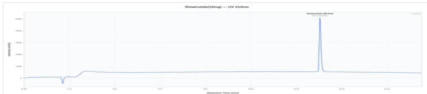
RETATRUTIDE 10mg - QPUSAR-0021: UV Chromatogram
